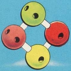
Model of Alpha Particle Made with Nuclear Spheres
